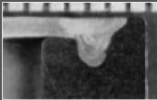
Figure 1d, weld cross-section of drop-in cover shown in figure 1c. The cover is 0.02" thick 4047 aluminum and the housing is 6061 aluminum. Weld penetration is 0.47".
