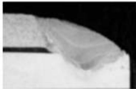
Figure 1f, weld cross- section of drop-in cover shown in figure 1e. Weld penetration is 0.025".
