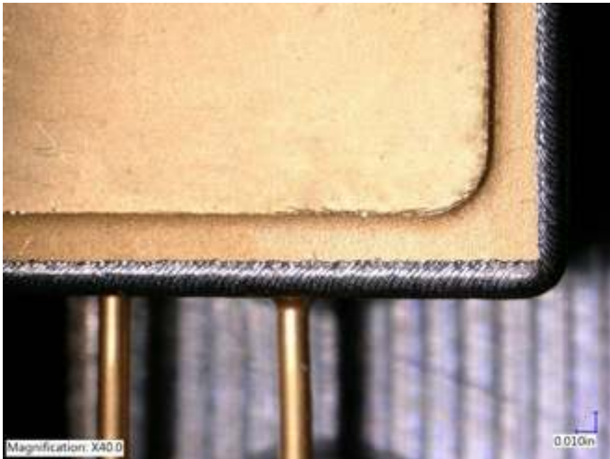
40x magnification of the finished weld.
