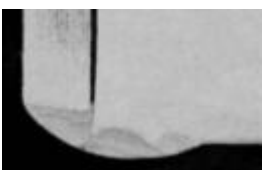
Figure 1b, cross-section of a butt weld in the stainless-steel relay in figure 1a, weld penetration is 0.008"
