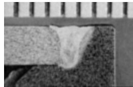
Figure 1h, weld cross-section of Beryllium-copper-to-copper butt weld. Weld penetration is 0.055".
