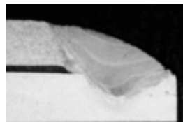
Figure 1g, weld cross-section of 4047-to-6061 aluminum fillet weld. The cover is 0.022" thick 4047 aluminum and the housing is 6061 aluminum. Weld penetration is 0.038".
