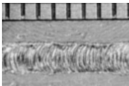
Figure 1e, top view of nickel-and gold-plated Kovar butt weld.
